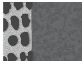
LaNiFe-geleding
